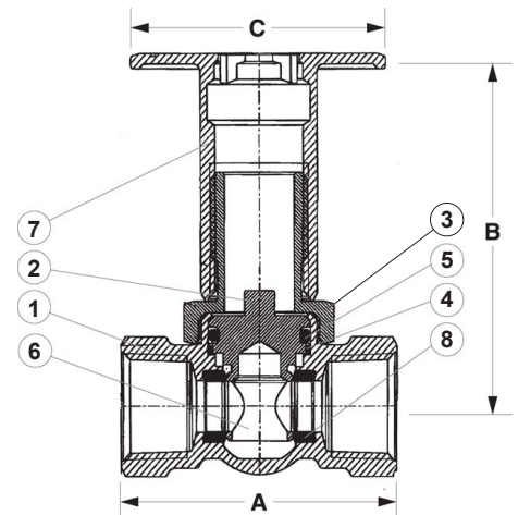
Pictured Model T-3500 Cut-away
